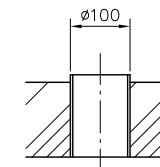
SLEEVE HOLE
